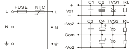
Figure 4: SLH**-10C** (Triple Output)
