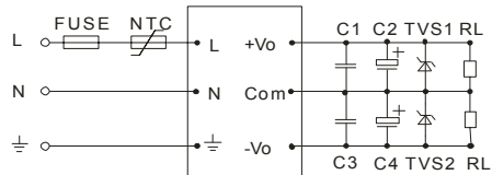
Figure 2: SLH**-10A** (Dual Output)
