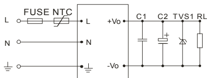
Figure 1: SLH**-10B** (Single Output)
