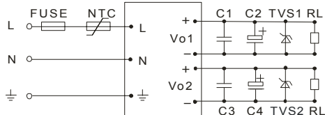
Figure 3: SLH**-10D** (Isolate Twin Output)
