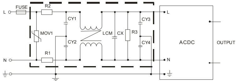
Figure 6: SLH05-25 series Recommended circuit for application require higher EMC standard (external circuit output same as above)
