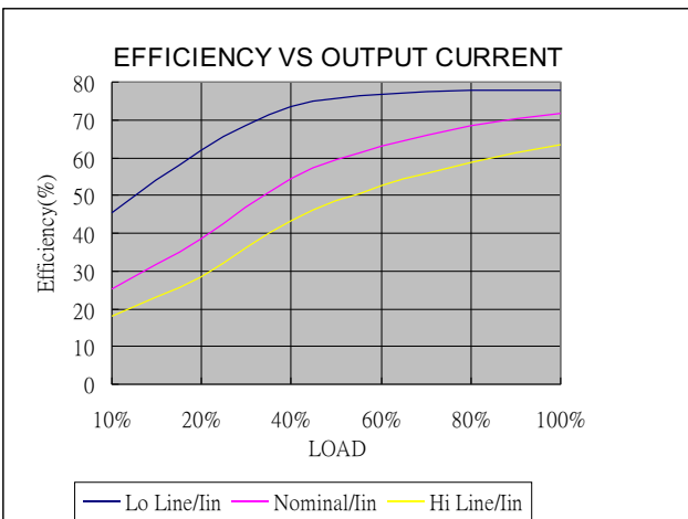
SRBW-123R3S2
